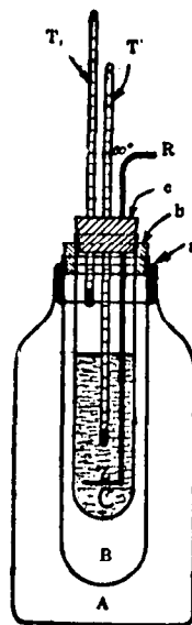
SETTING POINT APPARATUS
